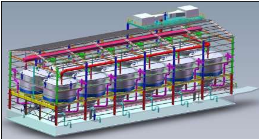
Process Plant Modelling
